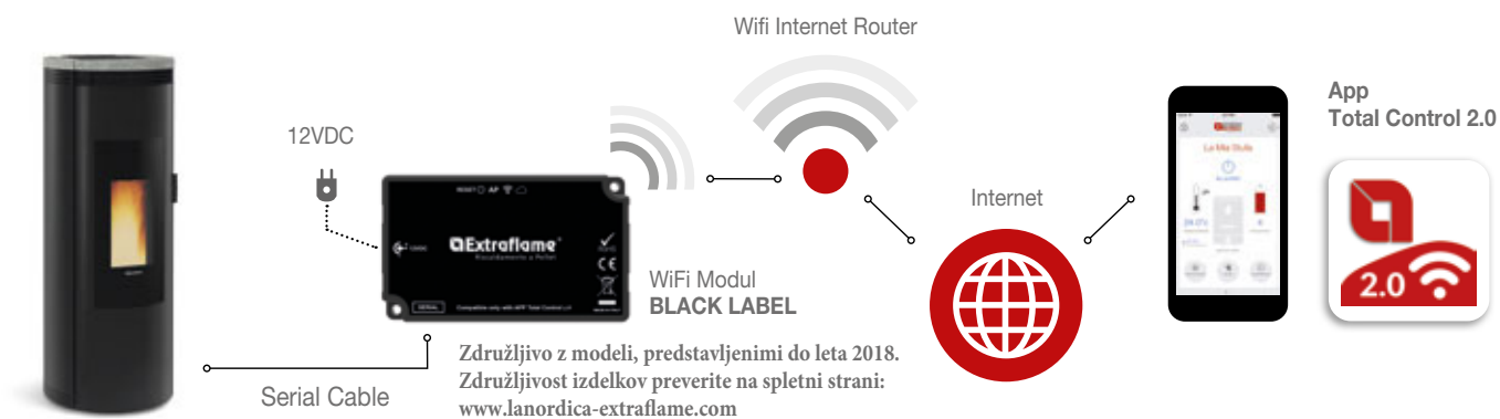
WiFi Modul diagram "BLACK LABEL" (B)
