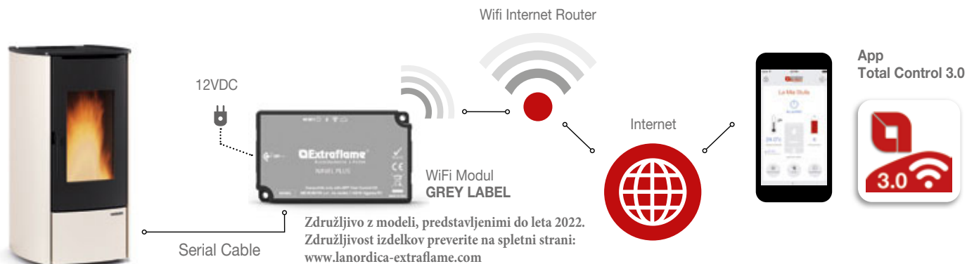
WiFi Modul diagram "GREY LABEL" (C)
